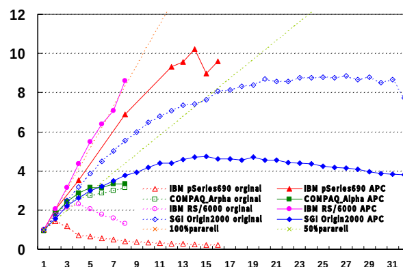
104.hydro2d (Hierarchical, cache optimize)
