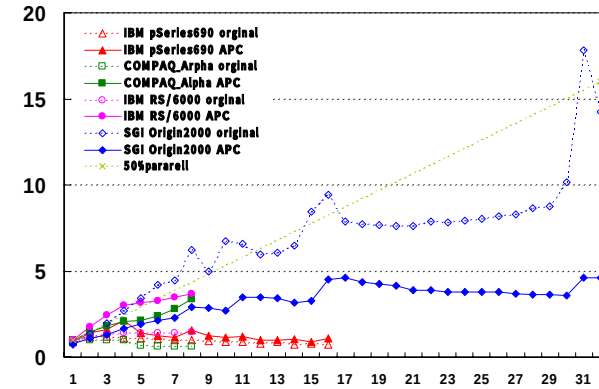
110.applu (Affine Transformation)
