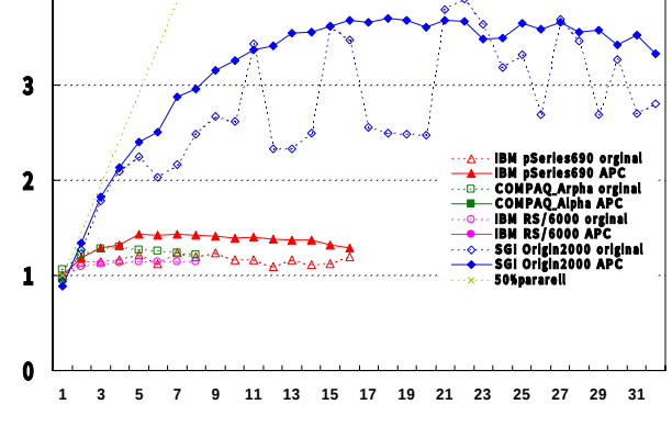
NPB2.3 SP-ClassA (Medium grain)
