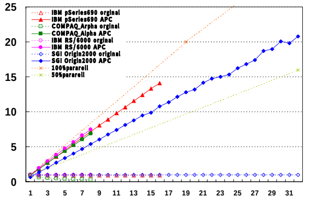
NPB2.3 EP-ClassA (Inter-procedural)
