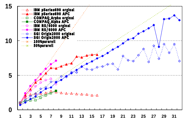
171. Swim (Hierarchical, cache optimize)
