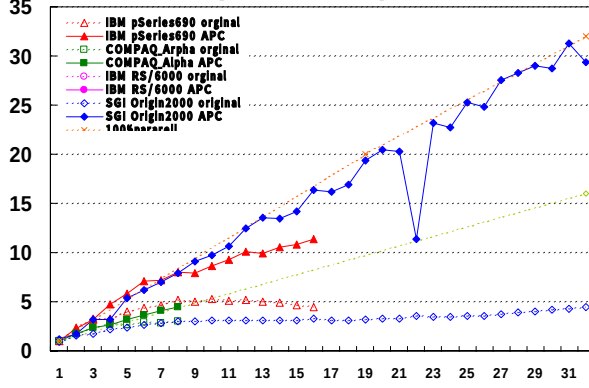
NPB2.3 CG-ClassB (First touch)
