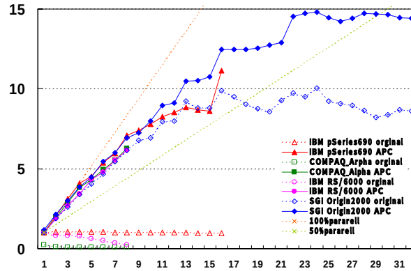
125. Turb3d (Hierarchical, Inter-procedural)
