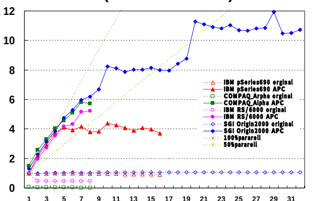
168. wupwise (Inter-Procedural)
