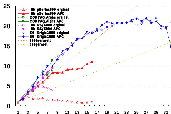
102.swim (Hierarchical, cache optimize)
